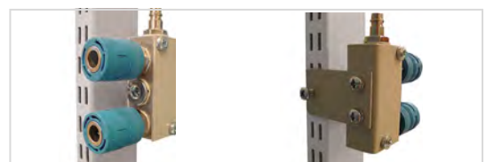
Distributor for compressed air
